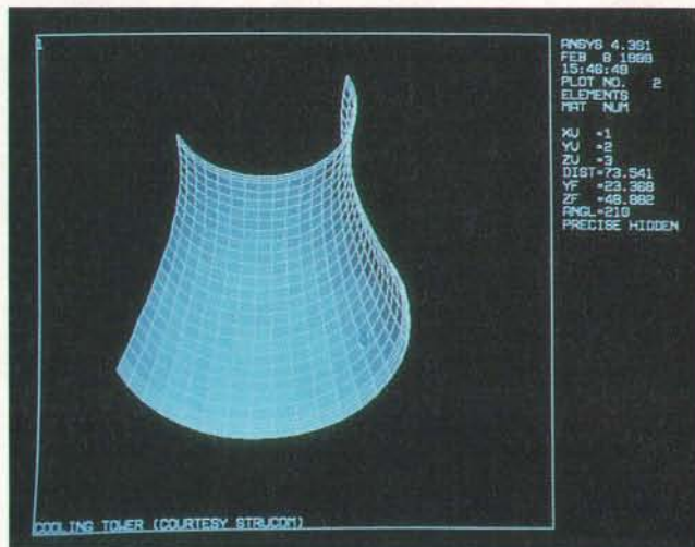
This Ansys-PC/Intro/Lin element display of a power plant cooling tower is made up of 520 quadrilateral shell elements and 140 three-dimensional elastic beam elements.
